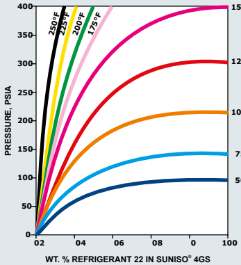
SOLUBILITY OF REFRIGERANT 22 IN SUNISO® 4GS as a function of Temperature and Pressure
